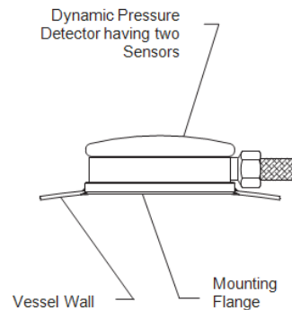
Dynamic Pressure Detector
