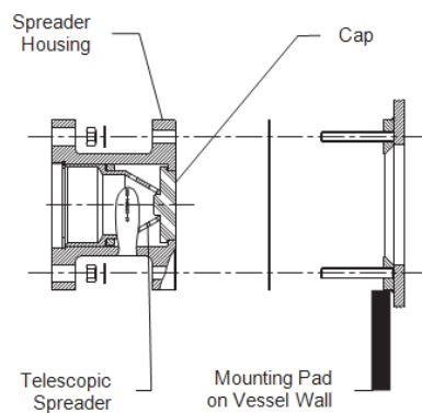
Extinguisher Flush Spreader
